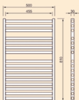
Elegance N 800/500
