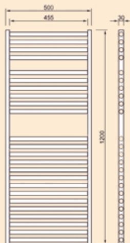
Elegance N 1200/500
