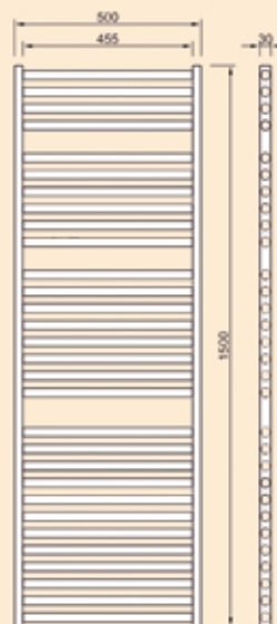
Elegance N 1500/500
